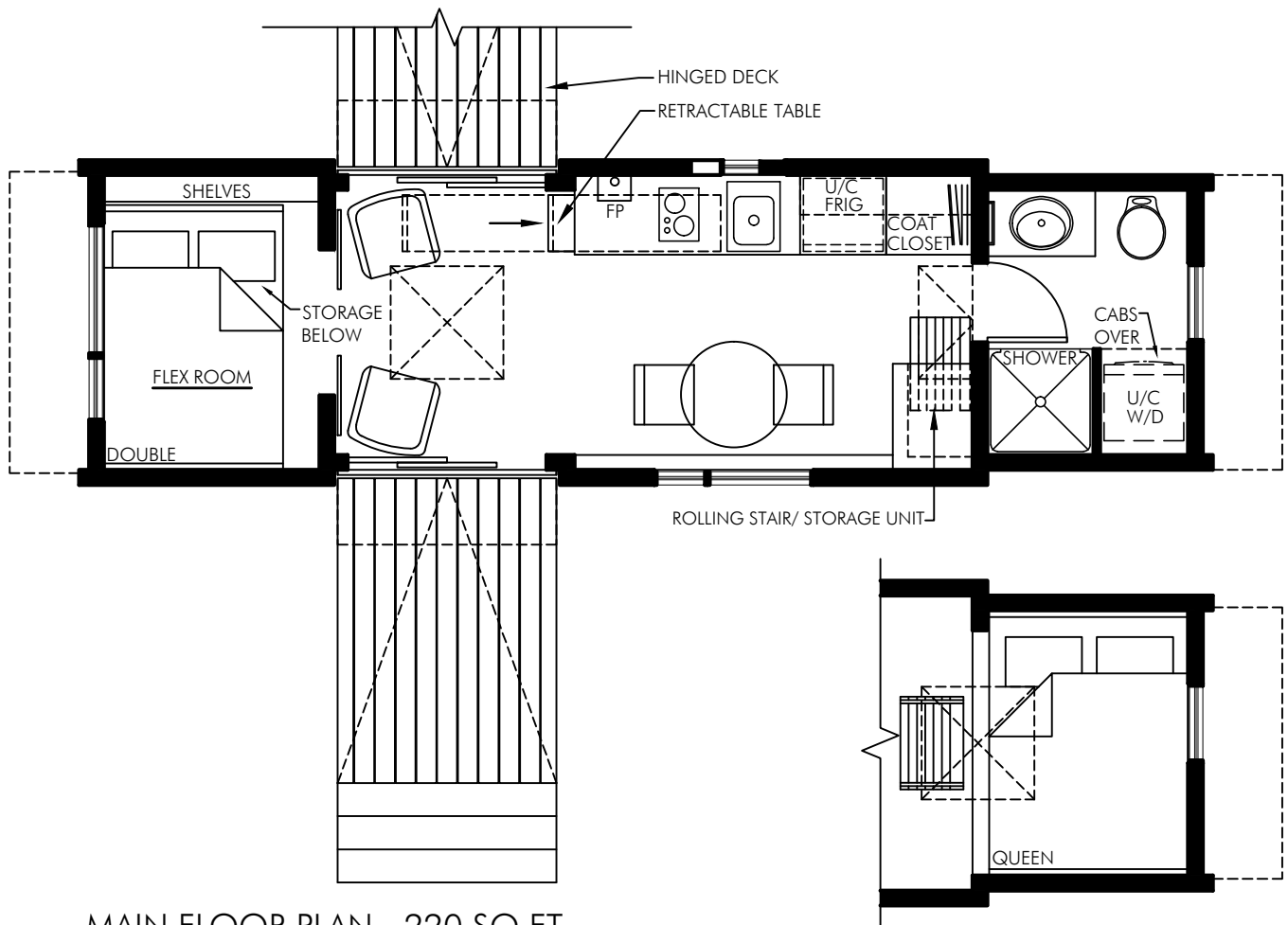
MAIN FLOOR PLAN - 220 SQ FT DRAGONFLY-28
