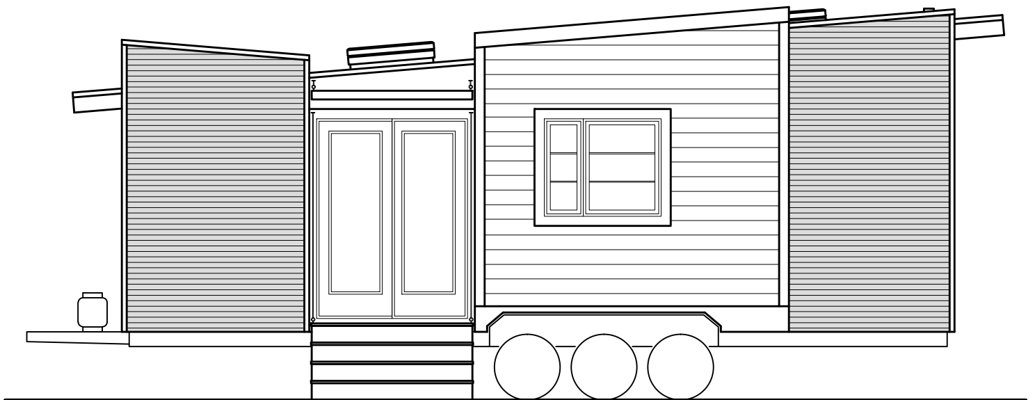
SIDE ELEVATION DRAGONFLY-28
